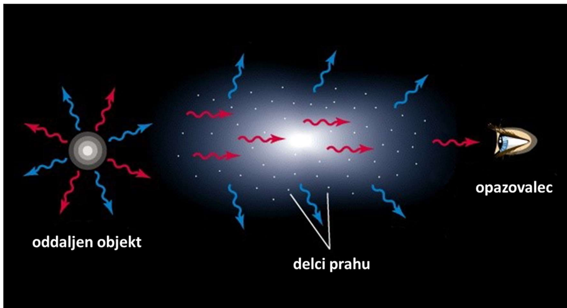
Slika 10: Ekstinkcija (prirejeno po https://scienceatyourdoorstep.com/2018/07/15/extinction-and-reddening-of-starlight/ )
